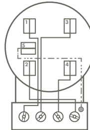
SSD-3W-5J-5T SHD-3W-5J-5T 4900-3W5J-5T-G2 FORM 12, 25S, 35
