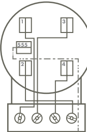
SSD-3W-5J SHD-3W-5J 4900-3W5J-G2 FORM 12, 25, 35
