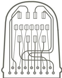
PTR-UNIVERSAL 15 JAW UNIVERSAL ADAPTER
