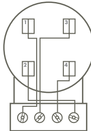
SSD-3W 4900-3W-G2 FORM 25
