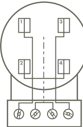
SSD-2W 4900-2W-G2 FORM 15
