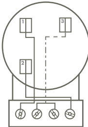
SSD-2W-2WM 4900-2W2WM-G2 FORM 15
